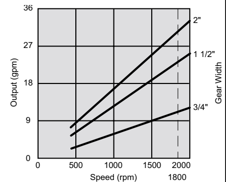
Dynaco G101 / G102 Performance curves
